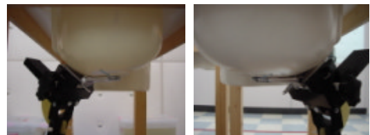
Fig. 17. Head SAR Test Setup
