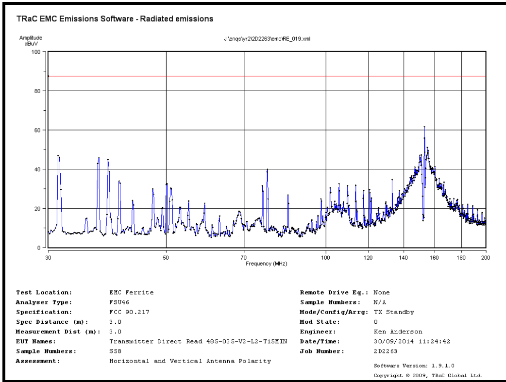
S58 TX 153.1MHz Radiated spurious emissions 30 MHz to 200 MHz
