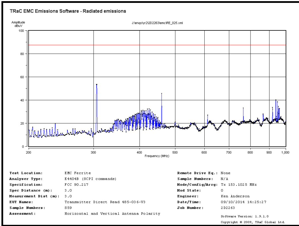
S59 TX 153.1MHz Radiated spurious emissions 200 MHz to 1000 MHz
