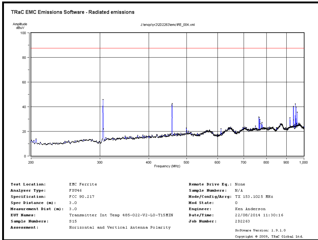
S15 TX 153.1MHz Radiated spurious emissions 200 MHz to 1000 MHz
