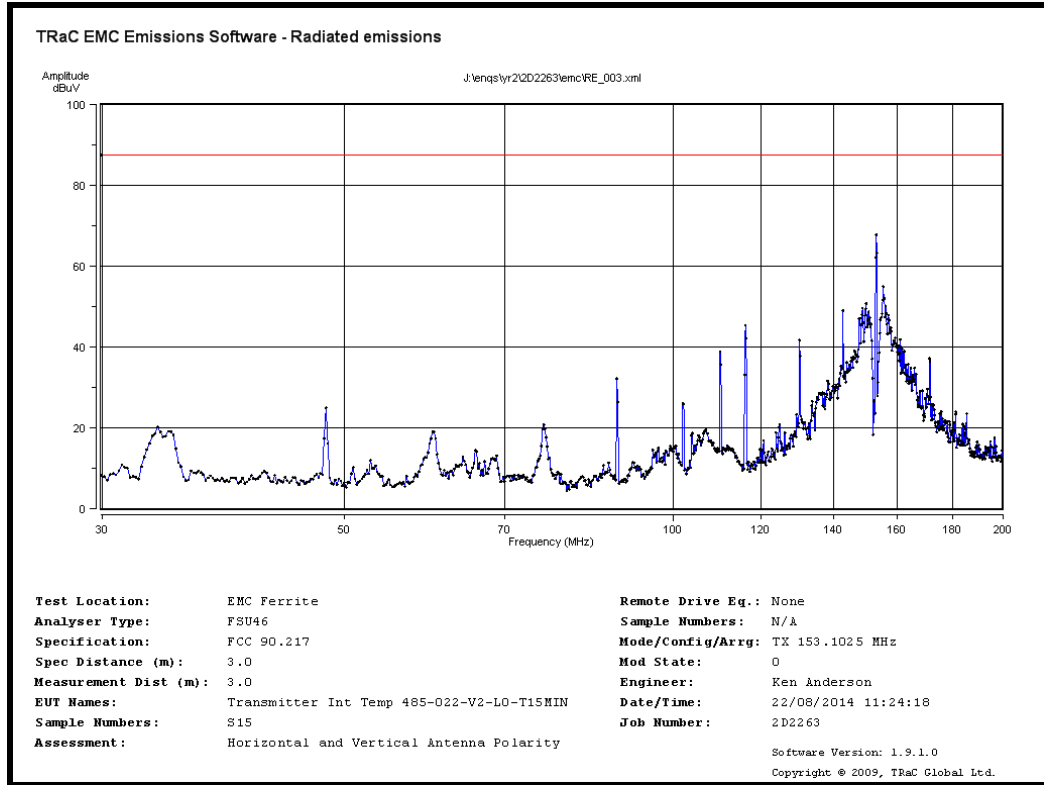
S15 TX 153.1MHz Radiated spurious emissions 30 MHz to 200 MHz
