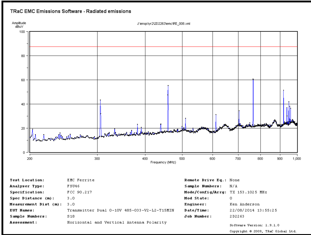
S18 TX 153.1MHz Radiated spurious emissions 200 MHz to 1000 MHz
