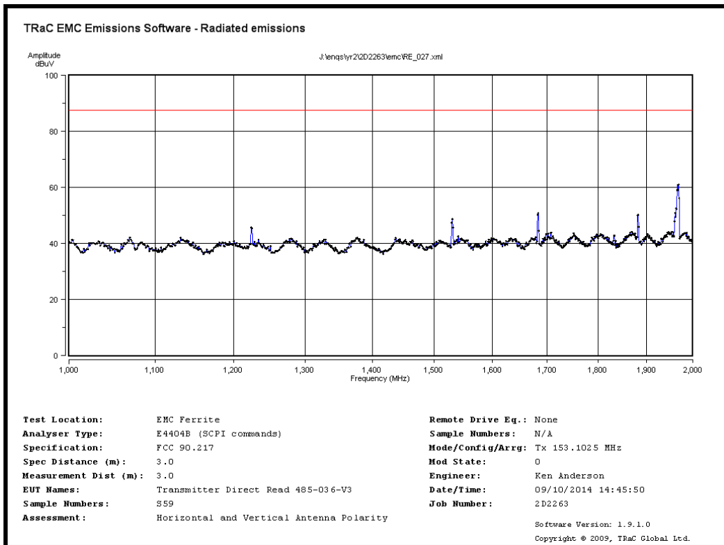
S59 TX 153.1MHz Radiated spurious emissions 1GHz to 2GHz
