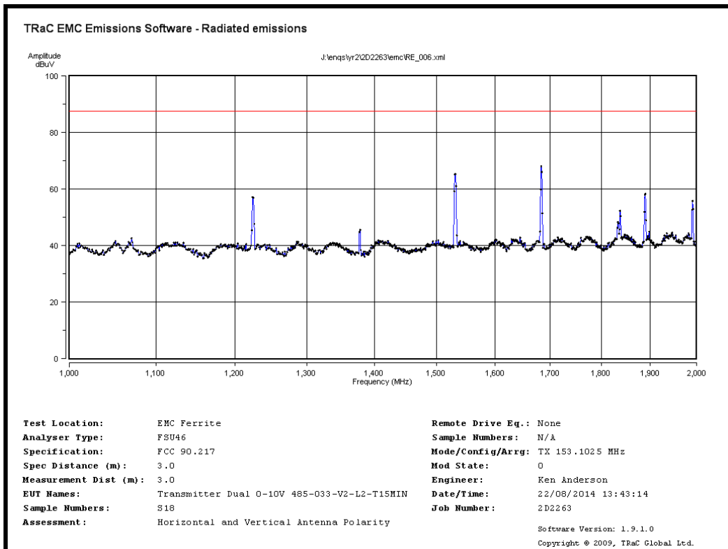
S18 TX 153.1MHz Radiated spurious emissions 1GHz to 2GHz
