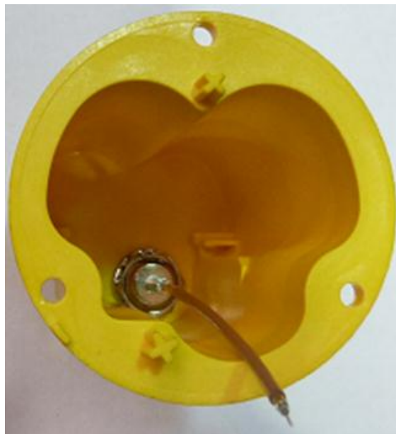
TNC connector mounted in battery housing.
