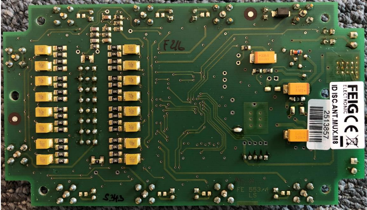
smartShelf Antenna
