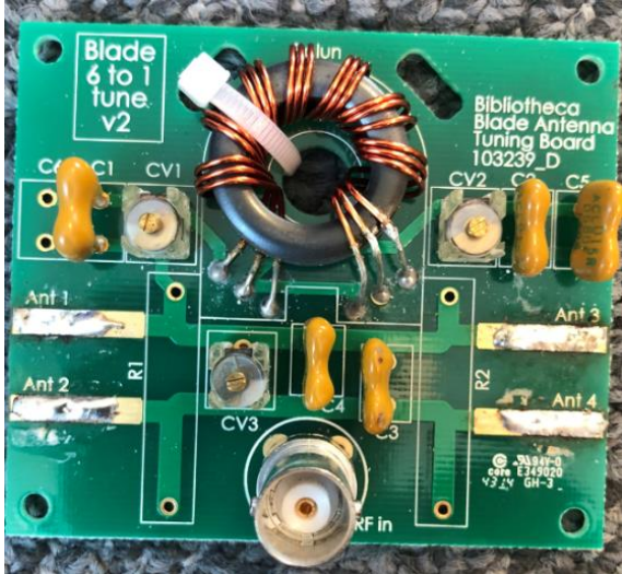
Antenna tuning board – Front
