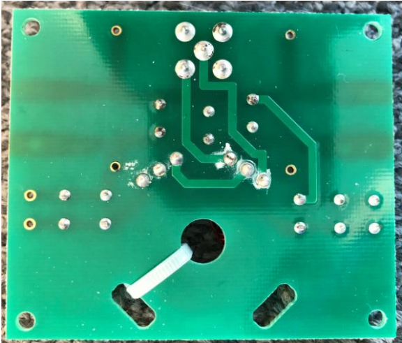
Antenna tuning board – Back
