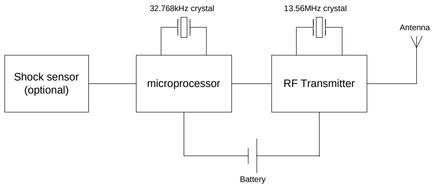
Figure 1: Tag_AAA block diagram
