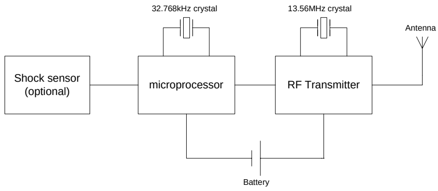
Figure 1: Tag_AA block diagram
