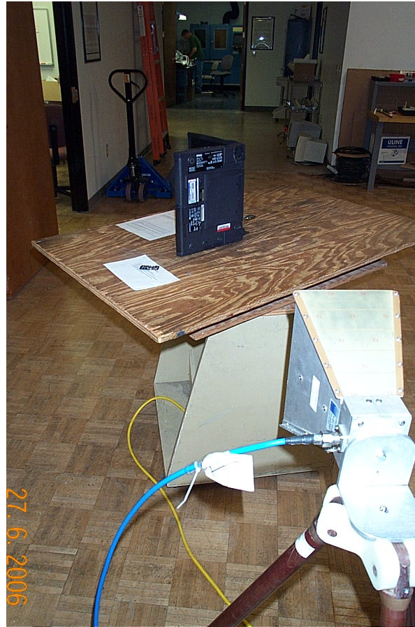
Figure 4, Peak Power, BW, Band Edge, Orientation 2
