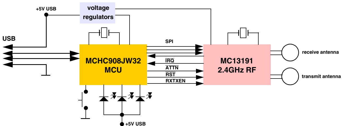
ZSTAR USB stick board block diagram
