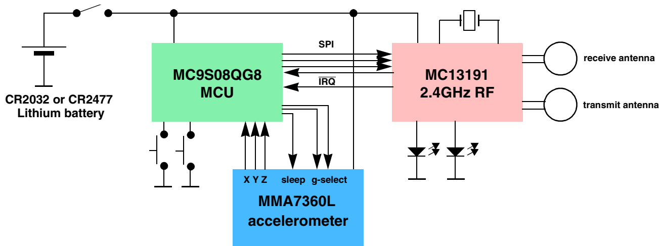
ZSTAR Sensor board block diagram
