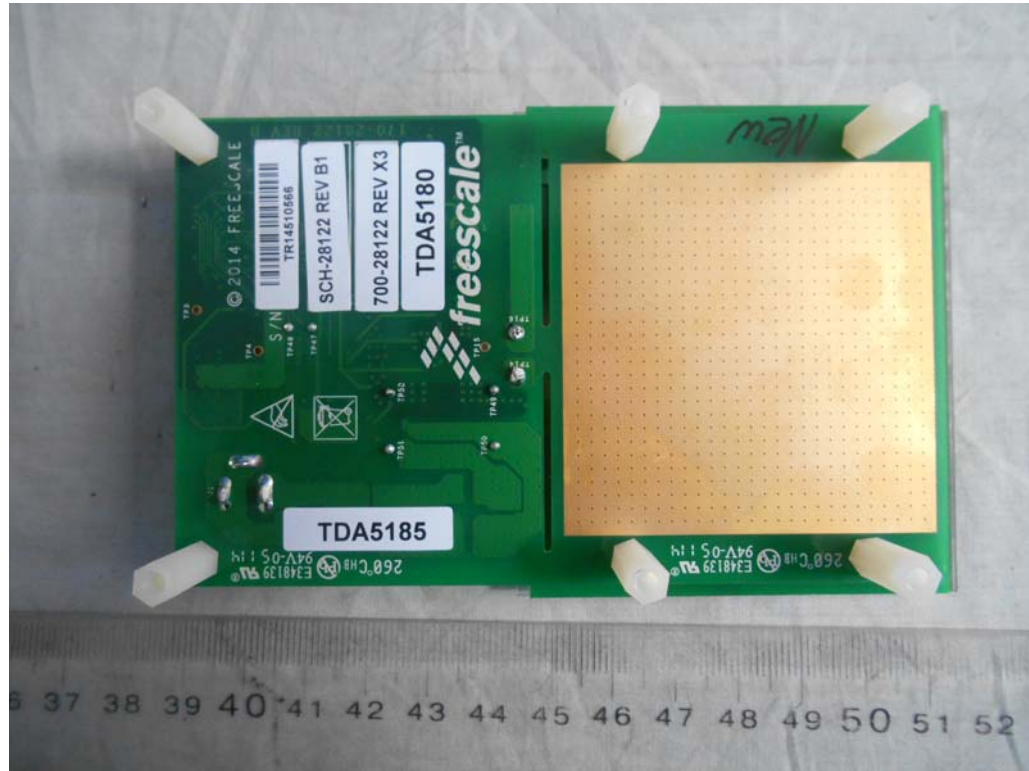
FIGURE 2 QI MEDIUM POWER WIRELESS CHARGER (M/N: WCT-15W1COILTX) BACK VIEW
