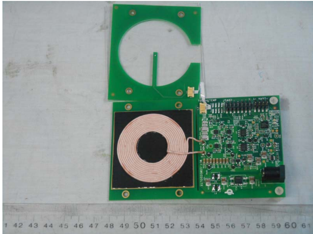
FIGURE 1 QI MEDIUM POWER WIRELESS CHARGER (M/N: WCT-15W1COILTX) COVER REMOVED
