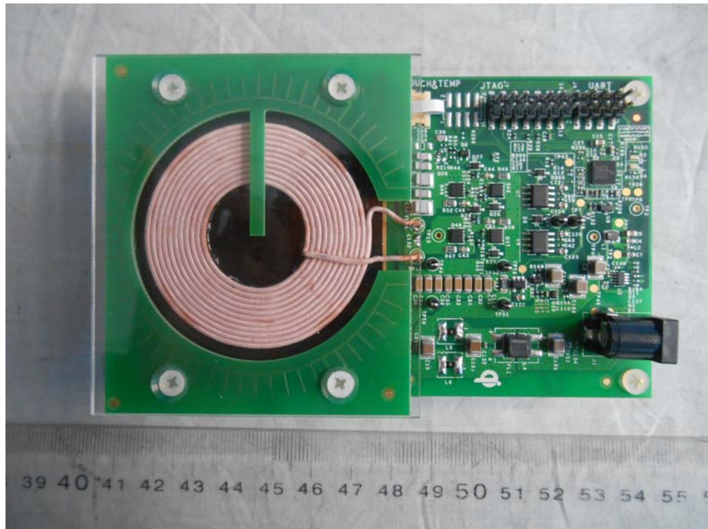
FIGURE 1 QI MEDIUM POWER WIRELESS CHARGER (M/N: WCT-15W1COILTX) GENERAL APPEARANCE (FRONT VIEW)
