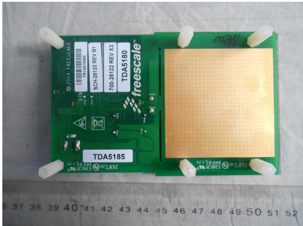
FIGURE 2 QI MEDIUM POWER WIRELESS CHARGER (M/N: WCT-15W1COILTX) GENERAL APPEARANCE (BACK VIEW)
