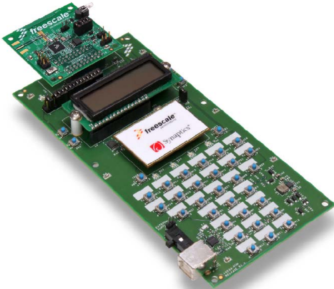
Figure 2-2. 1323x-MRB Mounted on the 1323x-RCM
