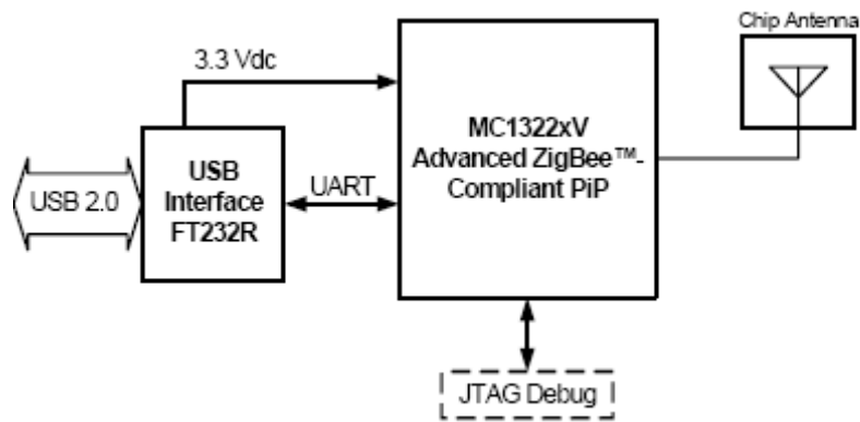
Figure 3-1. 1322x USB Dongle/Zniffer Block Diagram
