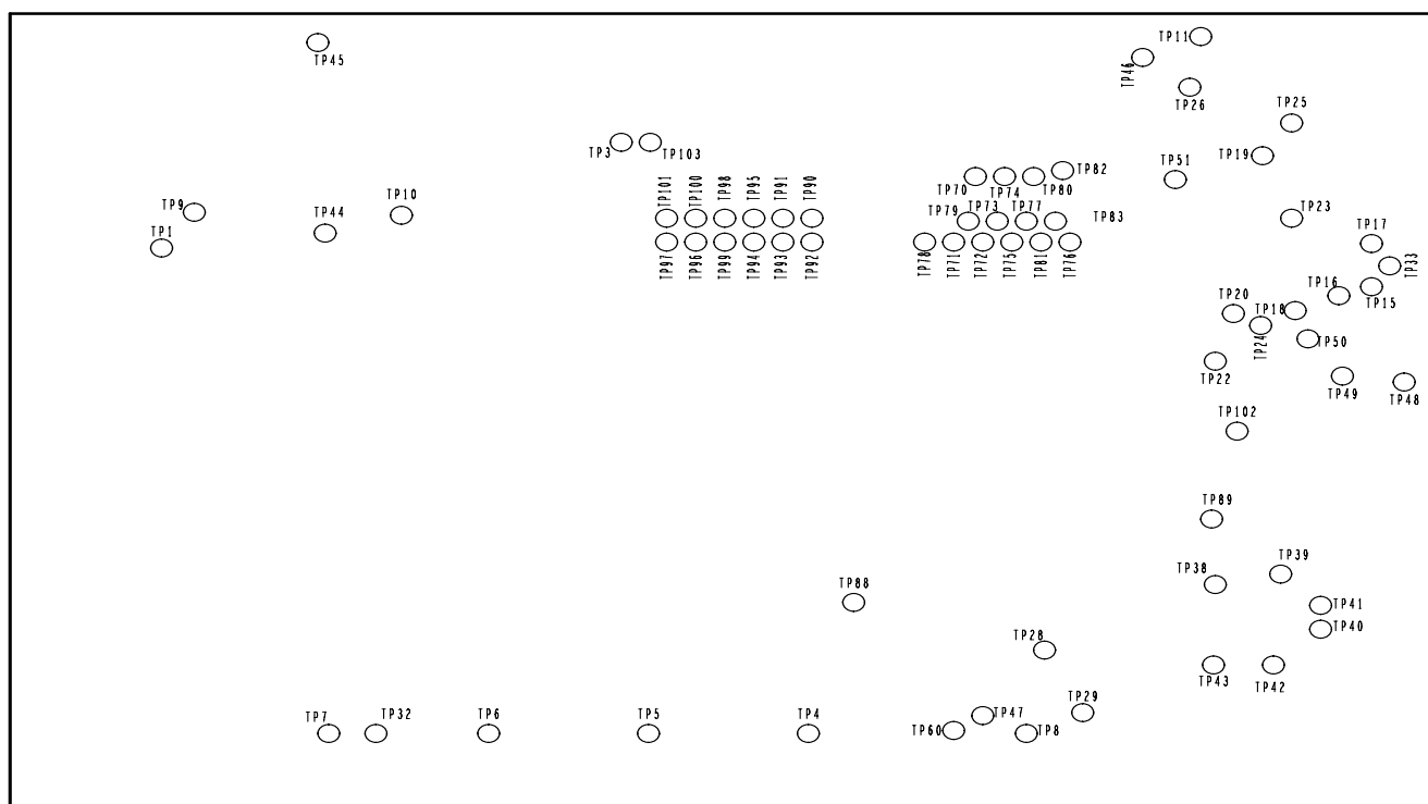
Figure 5-6. Network Node PCB Test Points (Bottom View)
