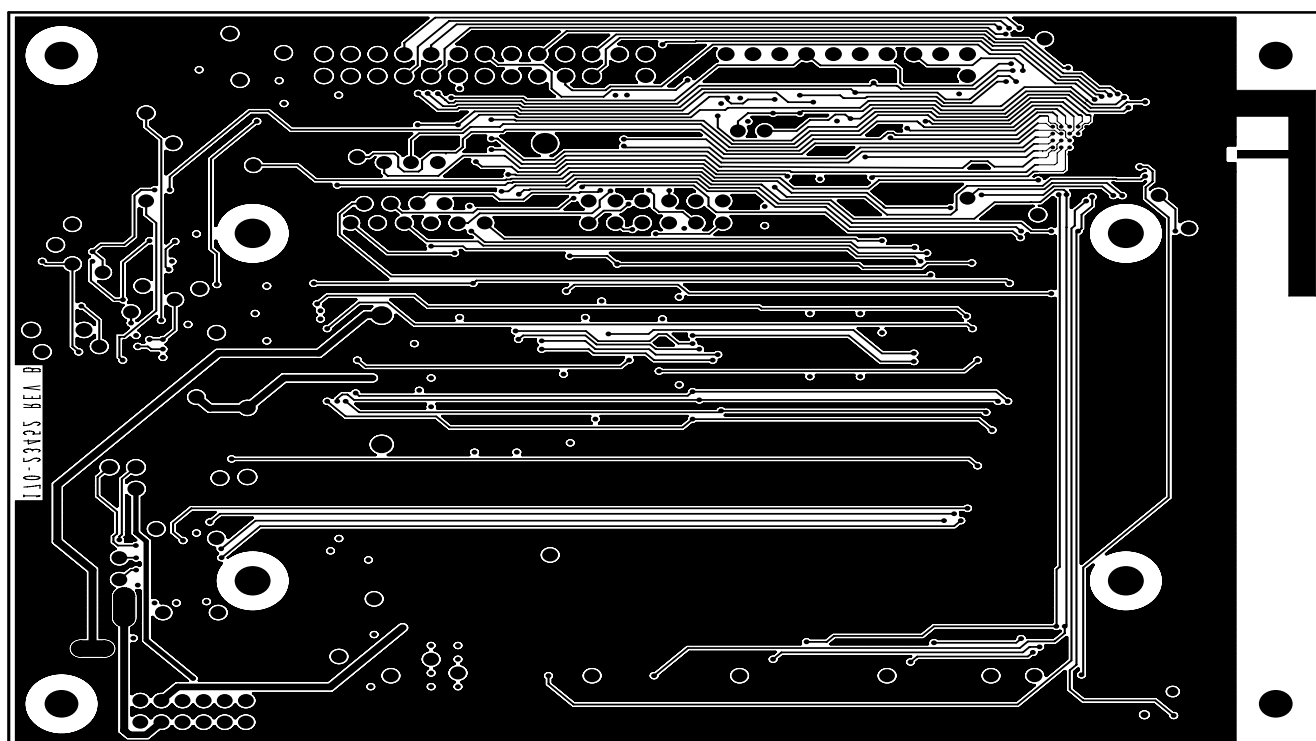
Figure 5-8. Network Node PCB Layout (Bottom View)
