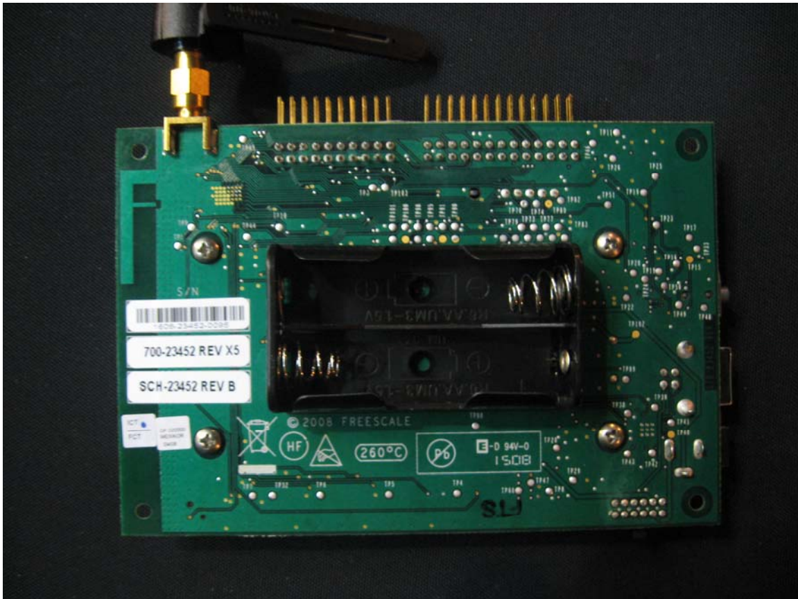
Bottom view of PCB
