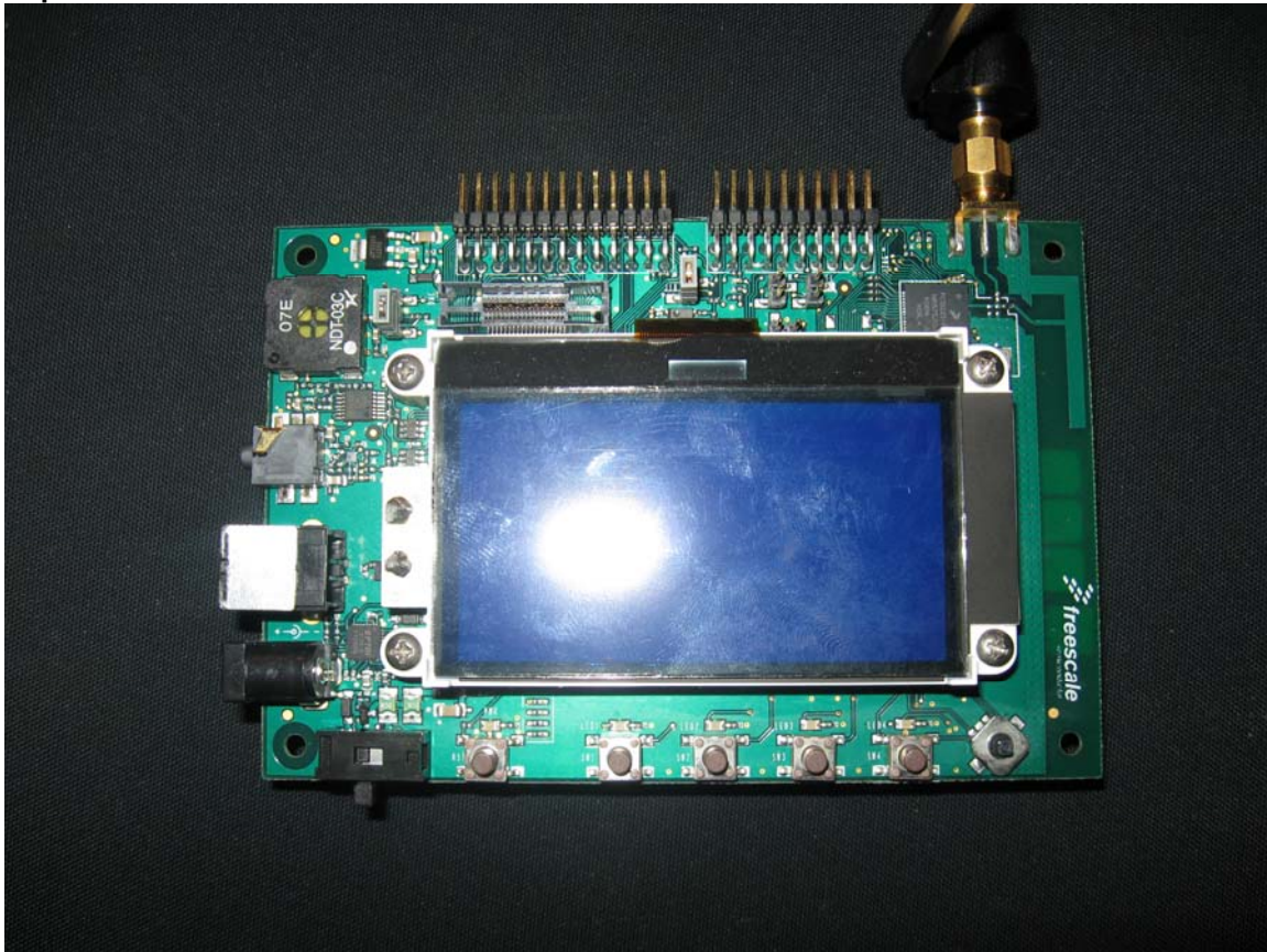
Top View Display Removed
