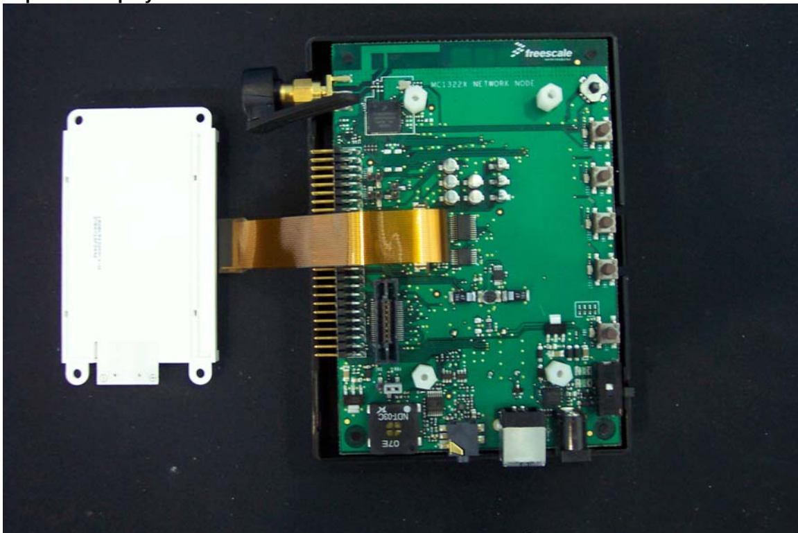
Top View Display Removed
