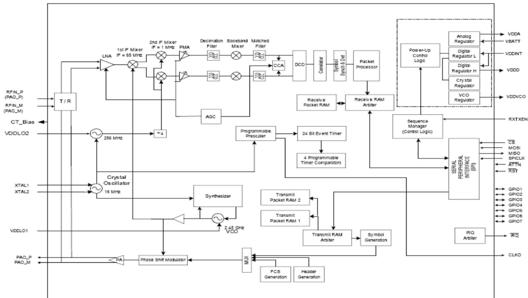
Figure 3-3. MC1320x Modem Block Diagram
