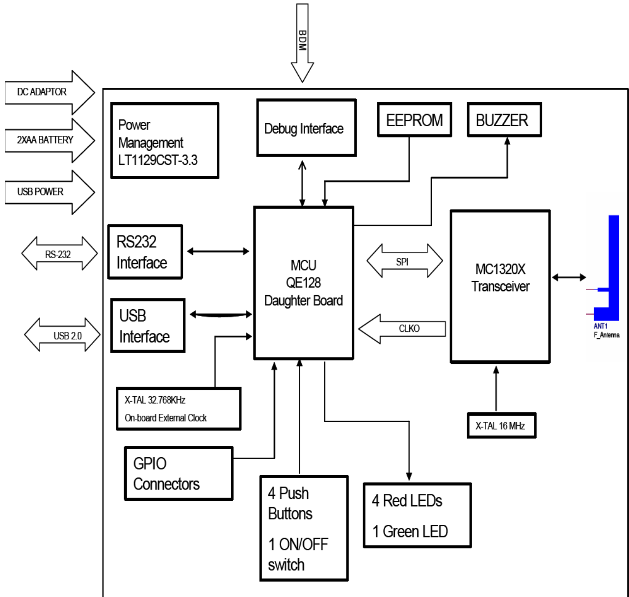
Figure 3-1. MC1320x and QE128 EVB Block Diagram
