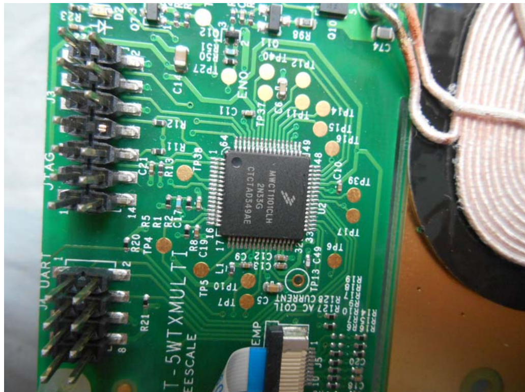
FIGURE 6 A28 MULTI-COIL WIRELESS CHARGER TRANSMITTER (M/N: WCT-5WTXMULTI) CHIP ON THE MAIN BOARD
