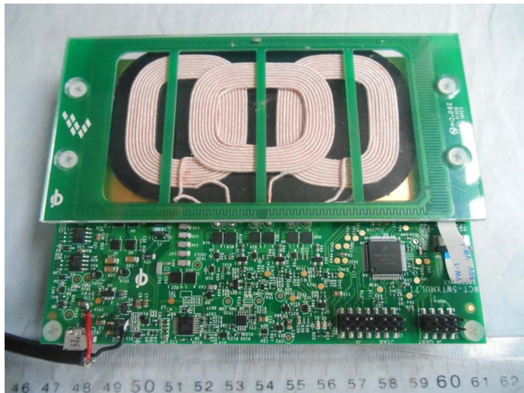
FIGURE 7 A28 MULTI-COIL WIRELESS CHARGER TRANSMITTER (M/N: WCT-5WTXMULTI) COIL
