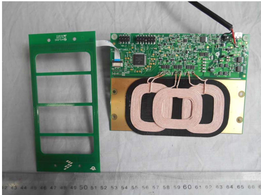
FIGURE 5 A28 MULTI-COIL WIRELESS CHARGER TRANSMITTER (M/N: WCT-5WTXMULTI) COVER REMOVED
