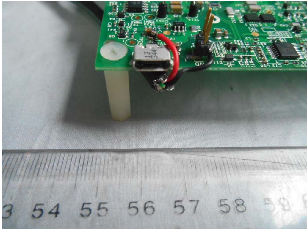
FIGURE 3 A28 MULTI-COIL WIRELESS CHARGER TRANSMITTER (M/N: WCT-5WTXMULTI) DC INPUT PORT
