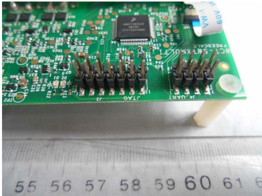
FIGURE 4 A28 MULTI-COIL WIRELESS CHARGER TRANSMITTER (M/N: WCT-5WTXMULTI) SIGNAL PORT
