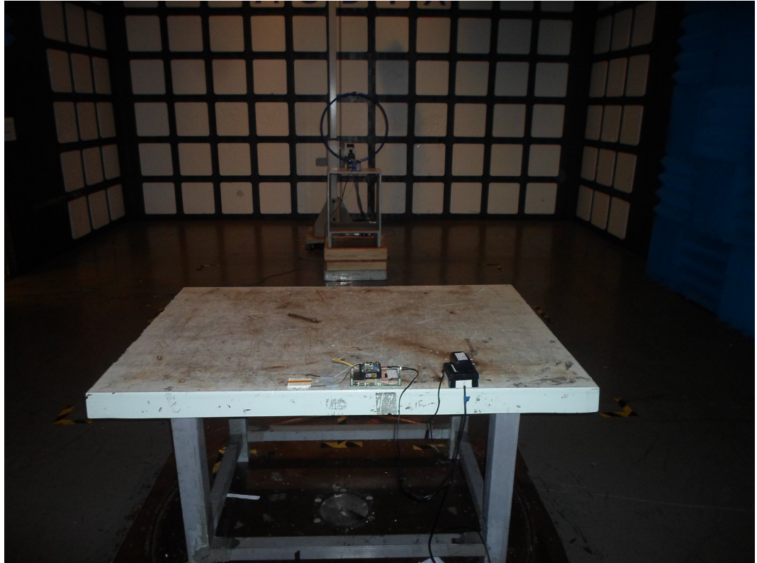
HORIZONTAL POLARIZATION
