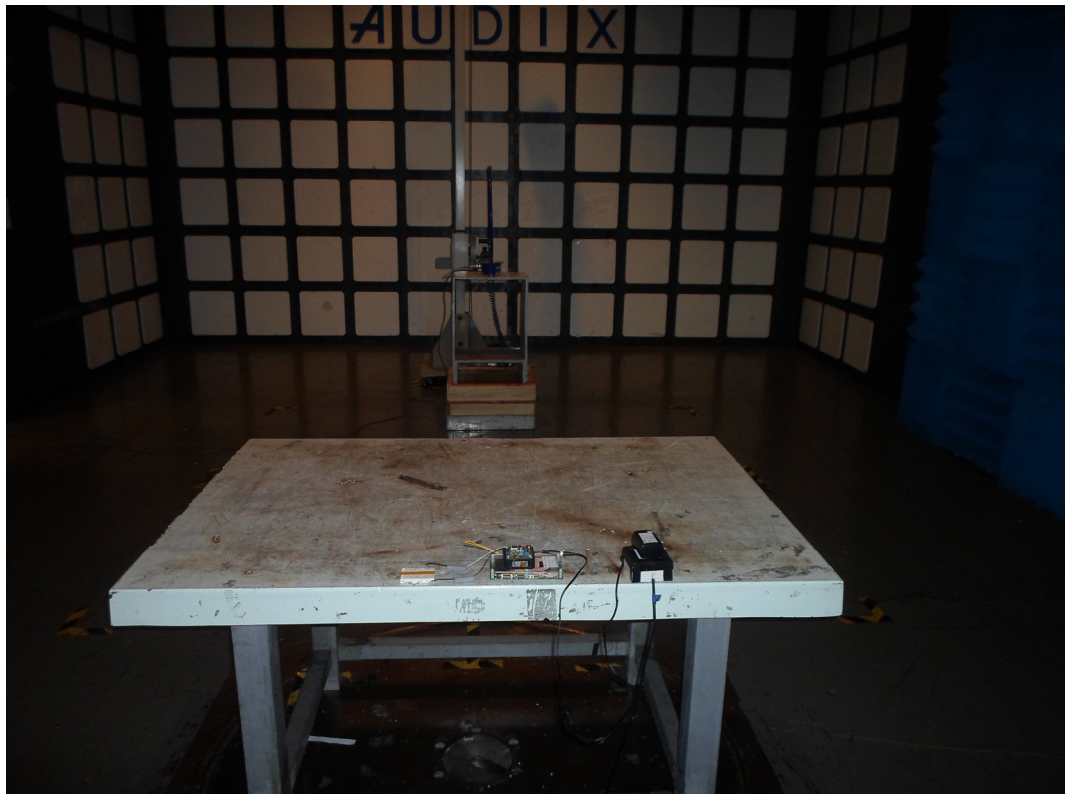
VERTICAL POLARIZATION
