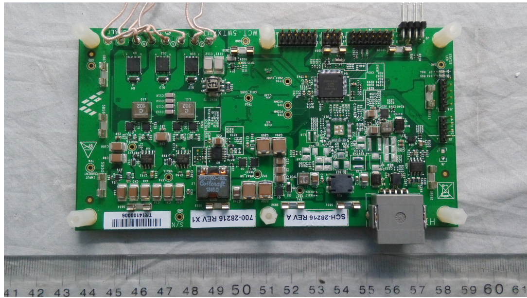
FIGURE 5 QI WIRELESS CHARGING TRANSMITTER (M/N: WCT-5WTXAUTO) MAIN BOARD (COMPONENT SIDE)
