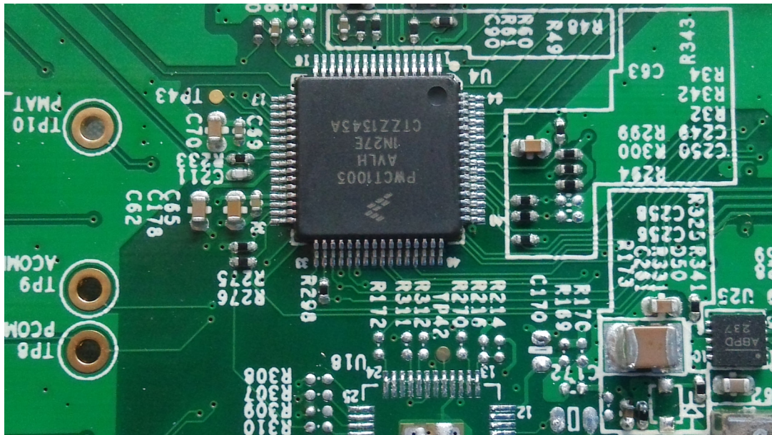
FIGURE 7 QI WIRELESS CHARGING TRANSMITTER (M/N: WCT-5WTXAUTO) CHIP ON MAIN BOARD
