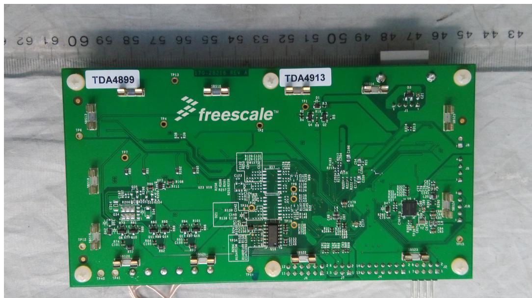
FIGURE 6 QI WIRELESS CHARGING TRANSMITTER (M/N: WCT-5WTXAUTO) MAIN BOARD (SOLDERED SIDE)
