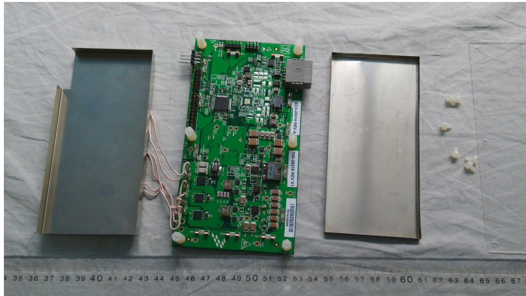
FIGURE 4 QI WIRELESS CHARGING TRANSMITTER (M/N: WCT-5WTXAUTO) COVER REMOVED
