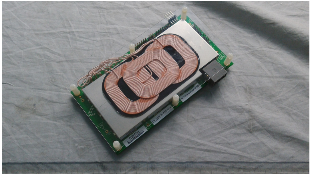
FIGURE 1 QI WIRELESS CHARGING TRANSMITTER (M/N: WCT-5WTXAUTO) GENERAL APPEARANCE (FRONT VIEW)
