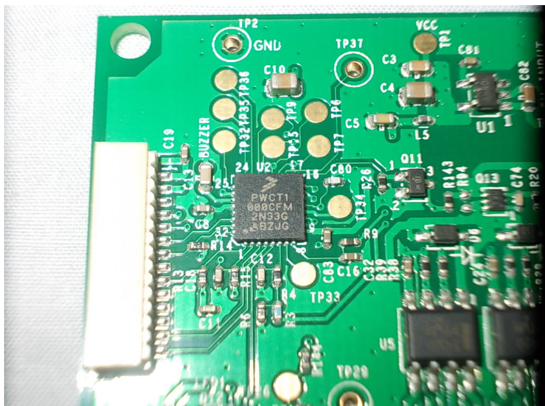
FIGURE 8 WIRELESS CHARGER TRANSMITTER (M/N: WCT-5W1COILTX) CHIP ON MAIN BOARD
