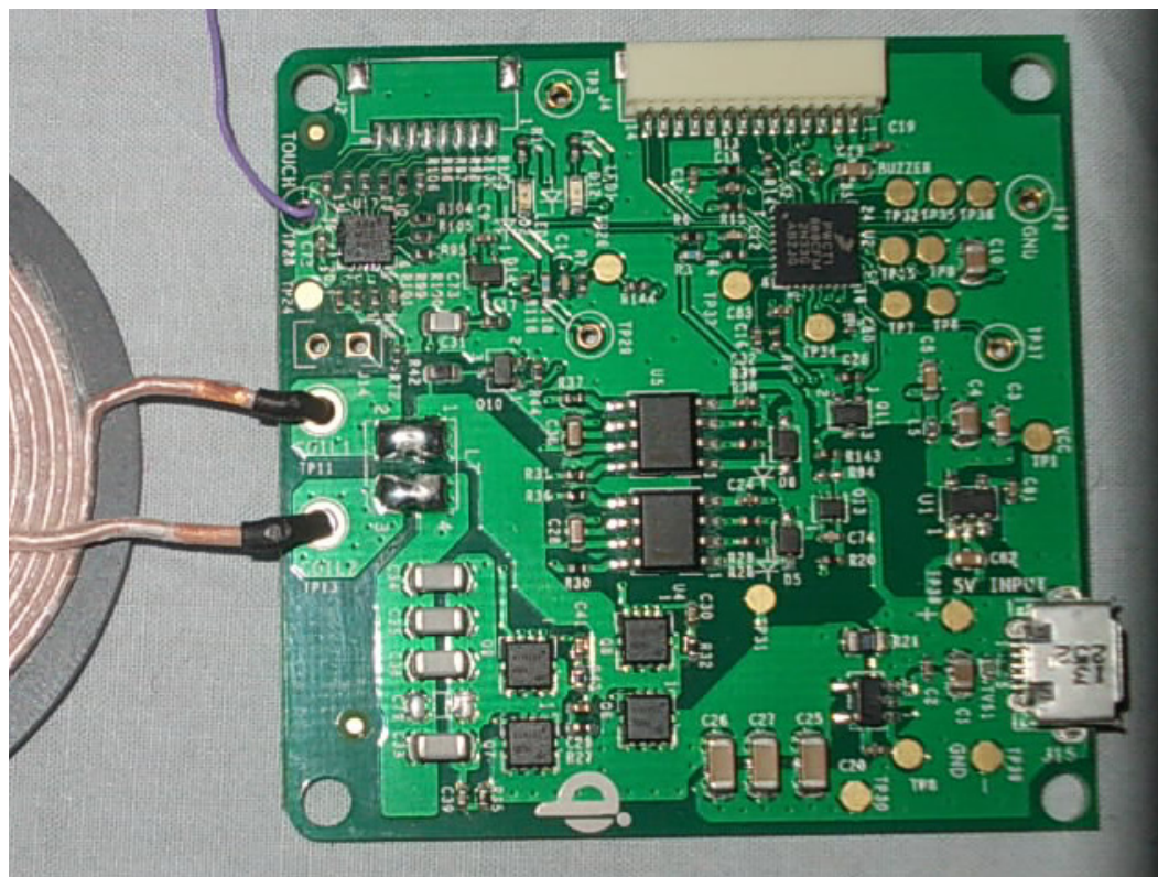
FIGURE 6 WIRELESS CHARGER TRANSMITTER (M/N: WCT-5W1COILTX) MAIN BOARD (COMPONENT SIDE)
