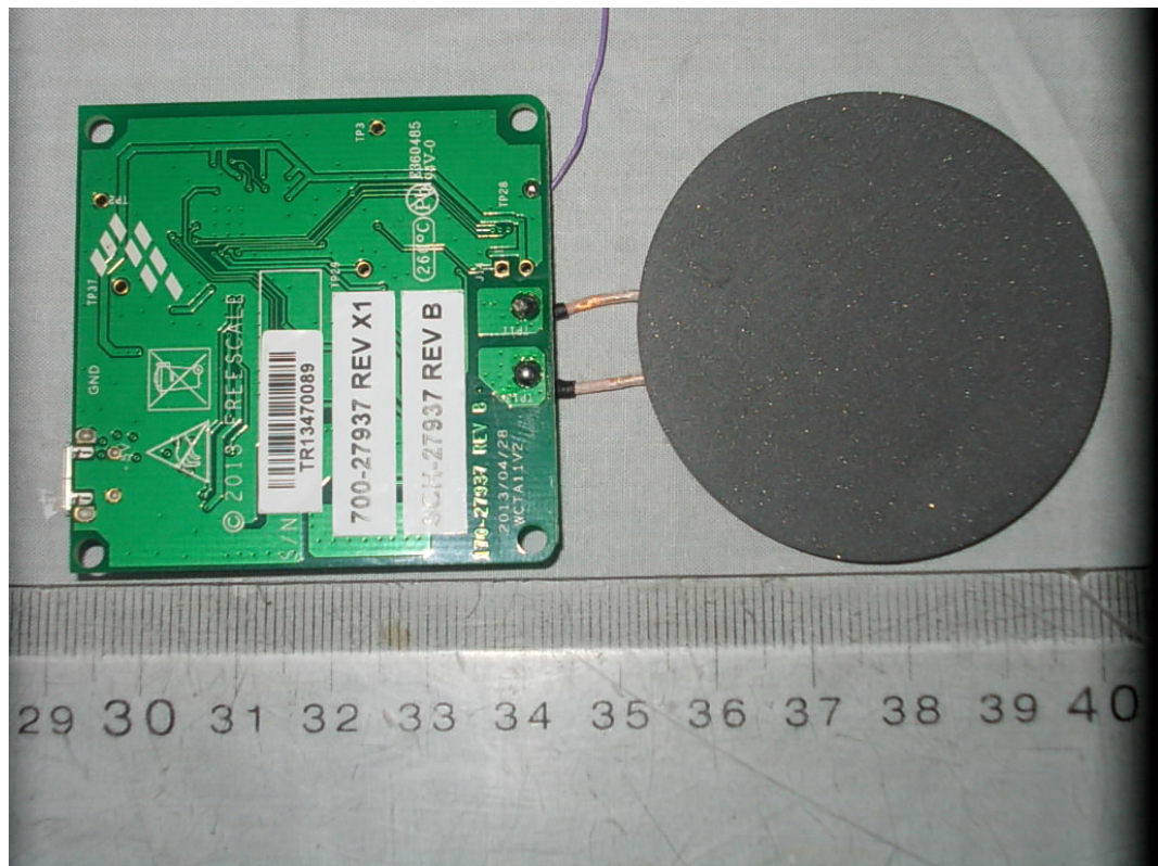
FIGURE 5 WIRELESS CHARGER TRANSMITTER (M/N: WCT-5W1COILTX) MAIN BOARD (BACK SIDE)
