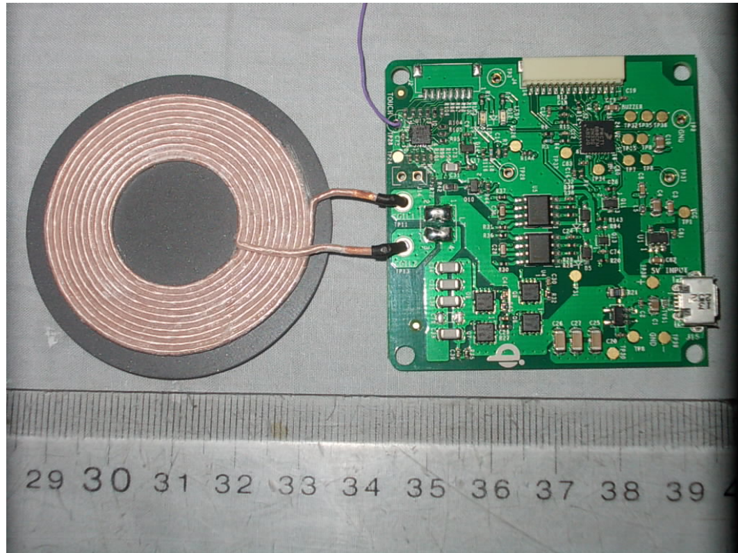
FIGURE 4 WIRELESS CHARGER TRANSMITTER (M/N: WCT-5W1COILTX) MAIN BOARD (FRONT SIDE)
