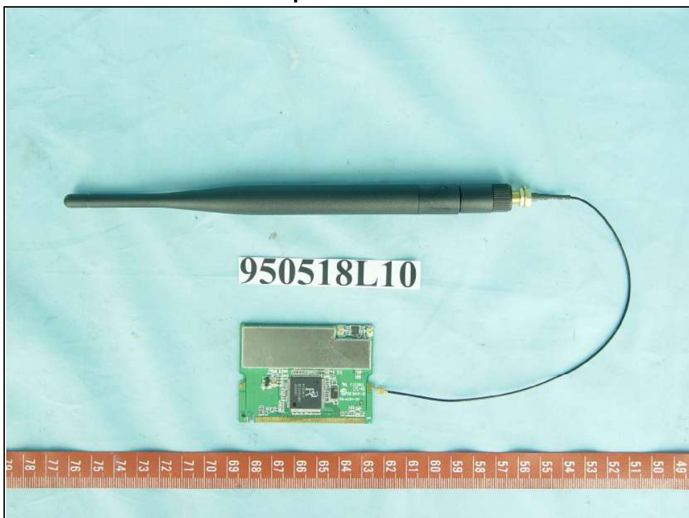
Dipole antenna
