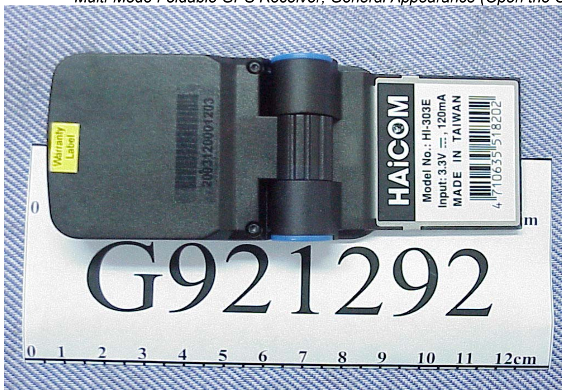
Figure 7 Multi-Mode Foldable GPS Receiver, General Appearance (Open the Cover)
