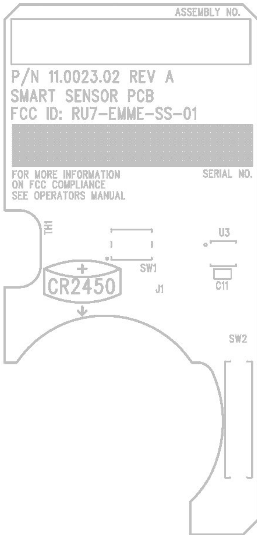
FCC ID Label Location on PCB Silkscreen (viewable with battery cover removed)
