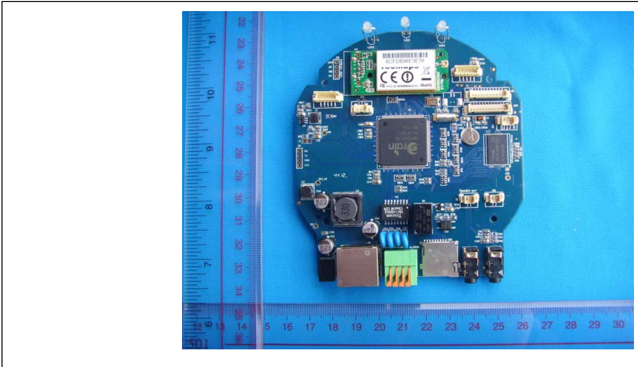
Details of: Main PCB
