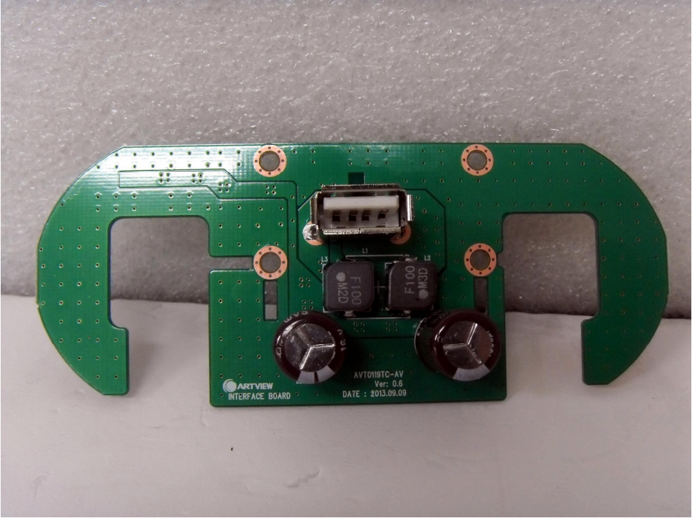
INTERFACE BOARD Photo_Front
