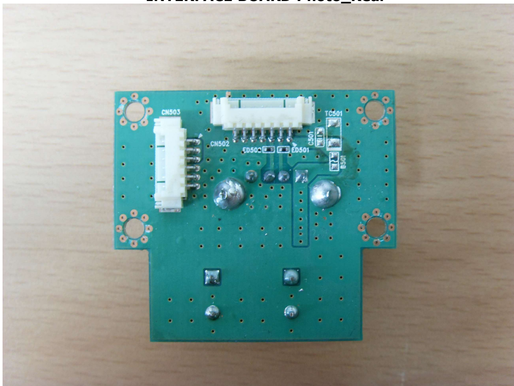
INTERFACE BOARD Photo_Rear
