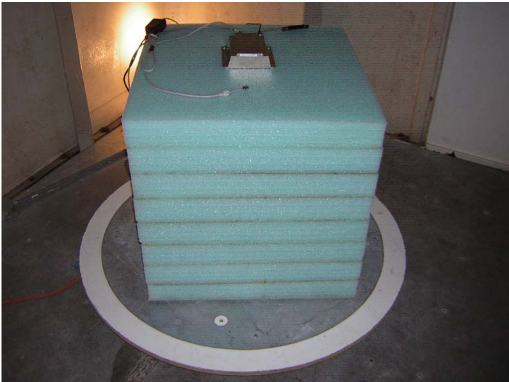
Radiated Emissions – Miltope antenna PN: 901167-2
