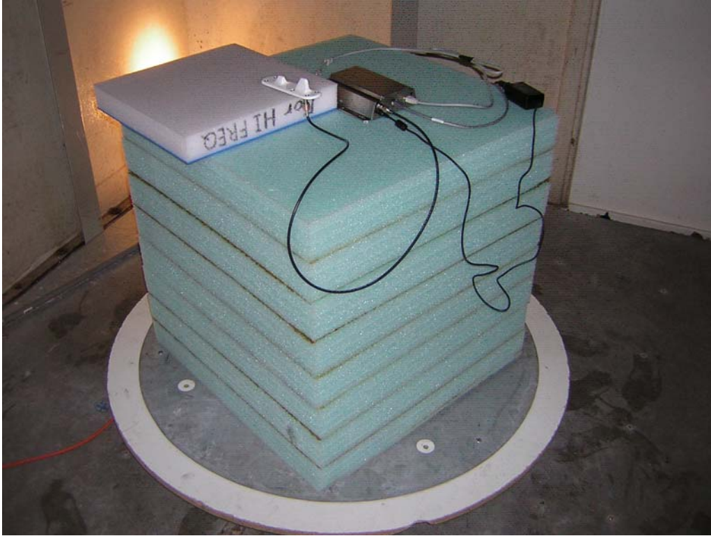
Radiated Emissions – Miltope antenna PN: 901563-2
