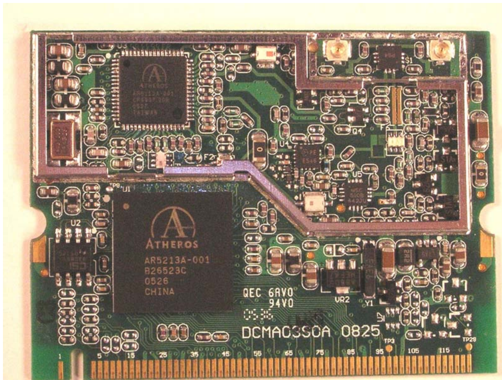
Top view of CM9-C1 with RF shielding removed
