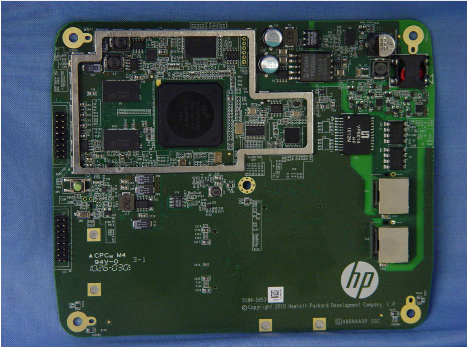
Main Assy with RF shield removed
