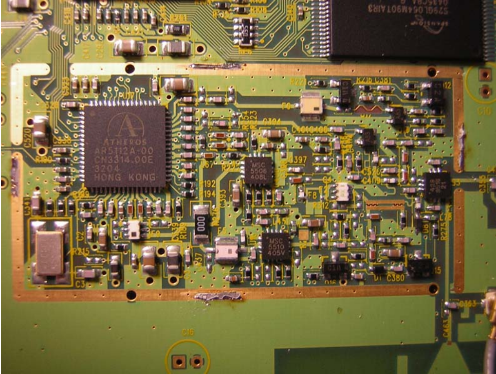
RF section without cover
