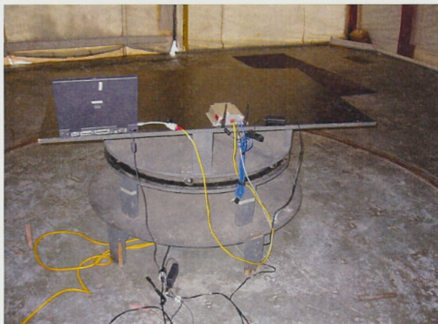
Radiated Spurious Test Setup, Back View
