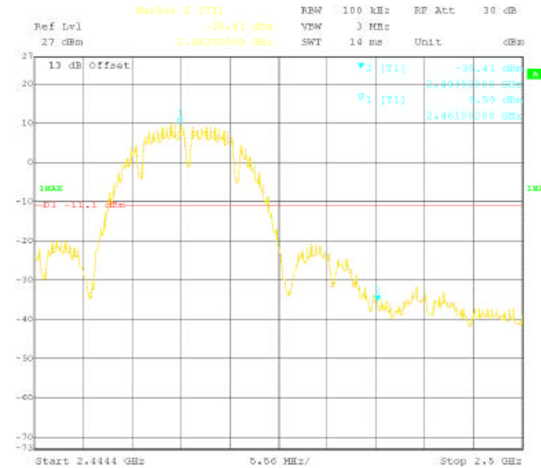
Band Edge Compliance (marker denotes upper band edge)
