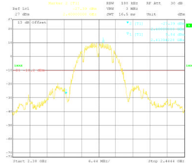
Band Edge Compliance (marker denotes lower band edge)
