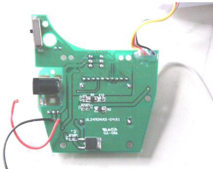
Main & RF board solder side
