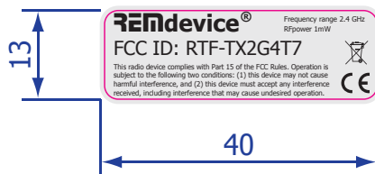
TX2G4T7 2.4 GHz transmitter
