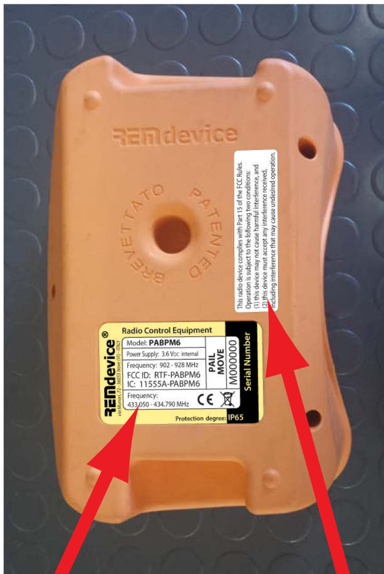
PABPM6 transmitter
