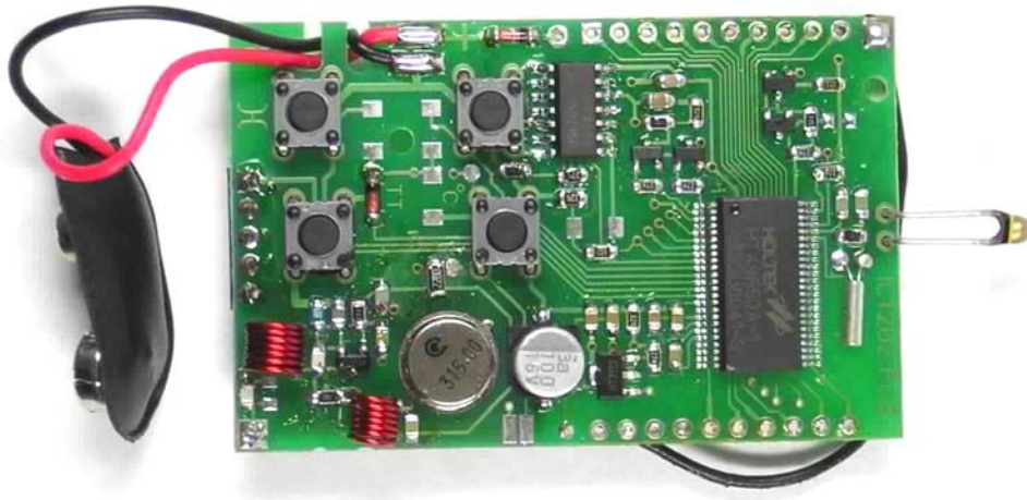
Internal Photo Part view of PCB
