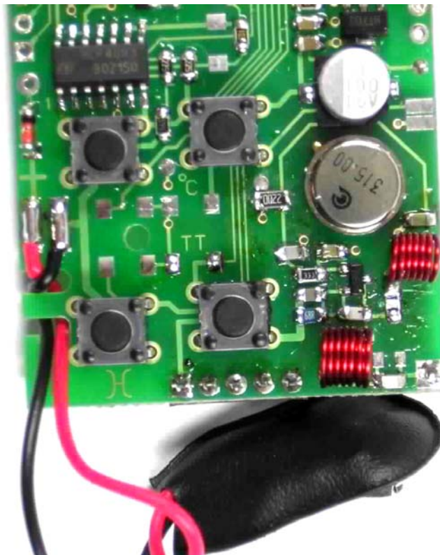
Internal Photo Part view of PCB
