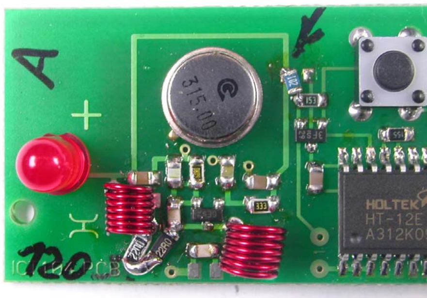
Internal Photo Part view of PCB
