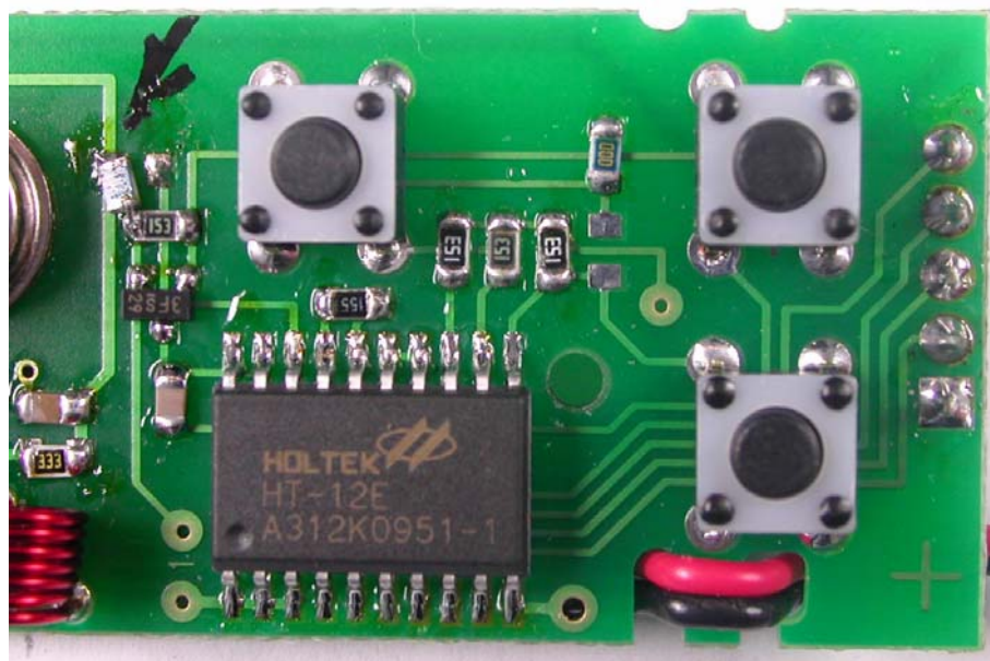
Internal Photo Part view of PCB
