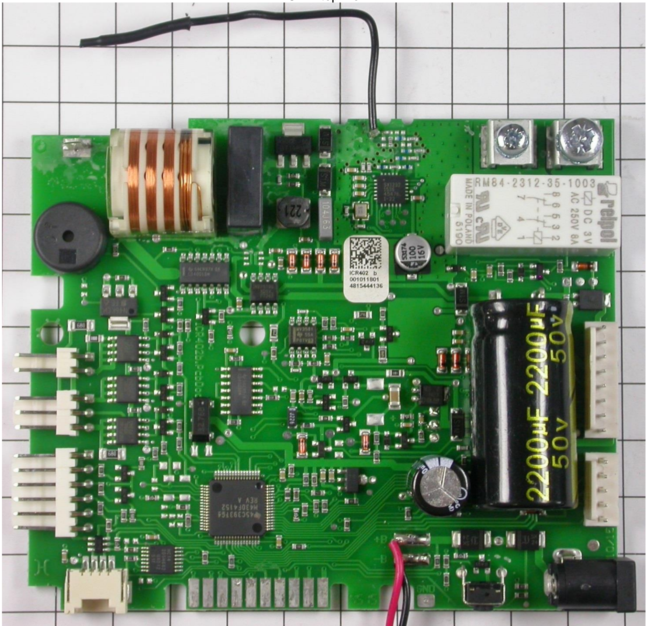
PCB – top view
