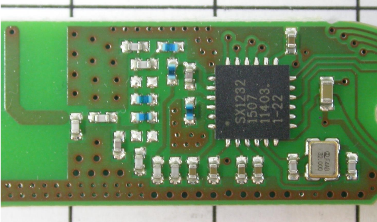
Detailed bottom view of the RF part
