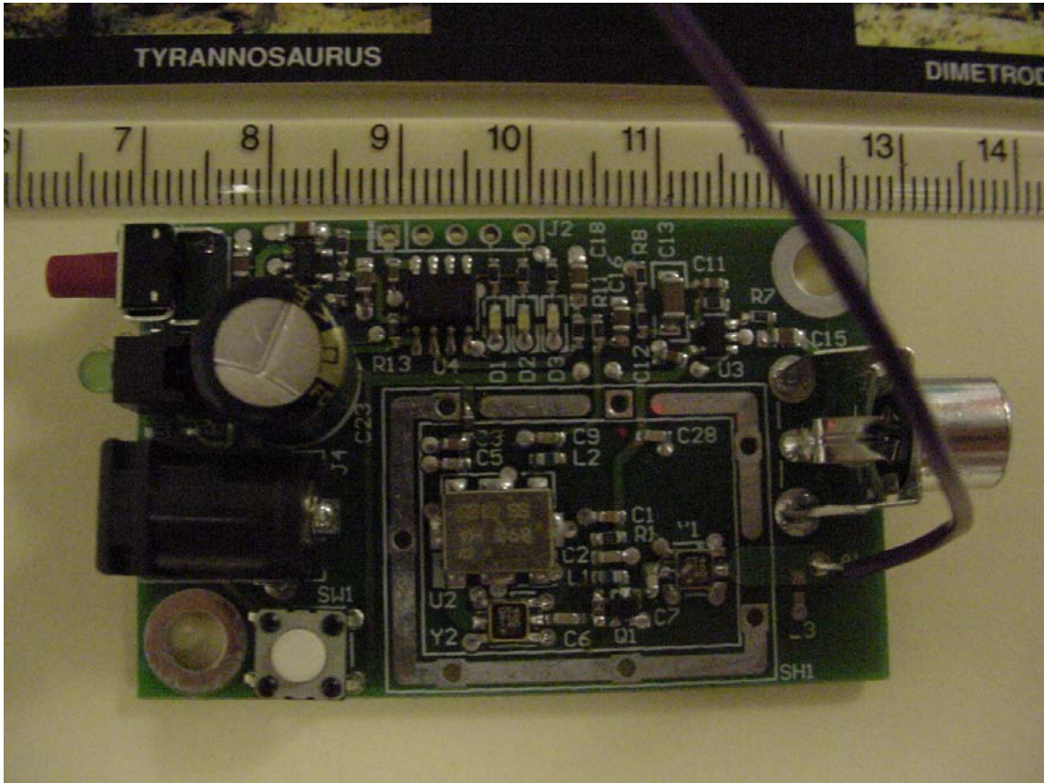
component side of PCB with RF shield removed
