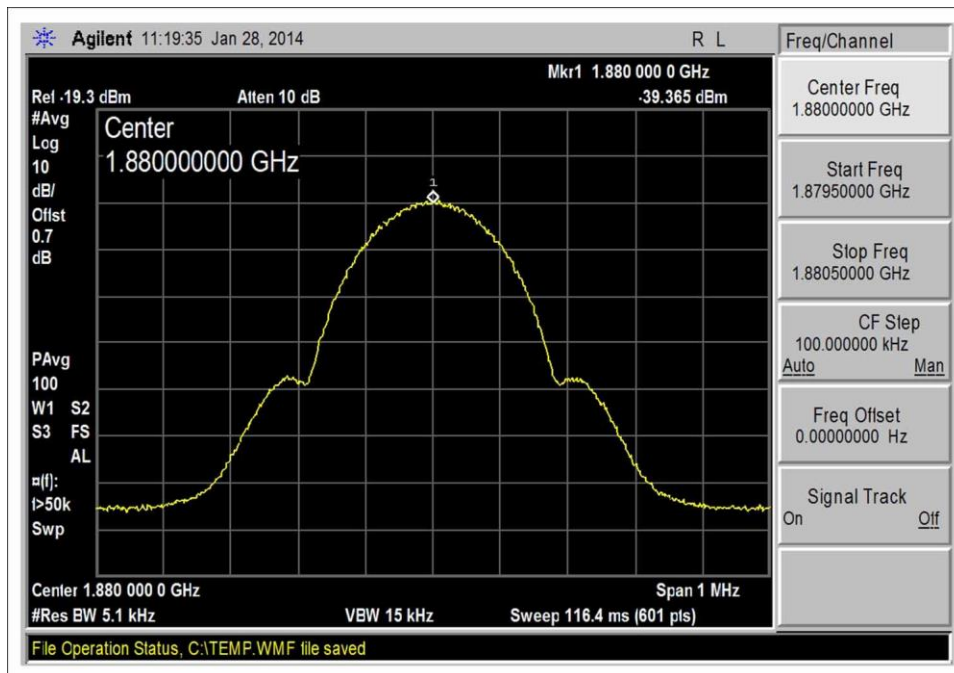
GSM_UL 1850-1910_Input
