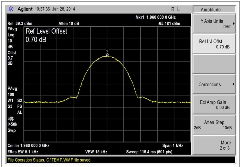
GSM_DL 1930-1990_Input
