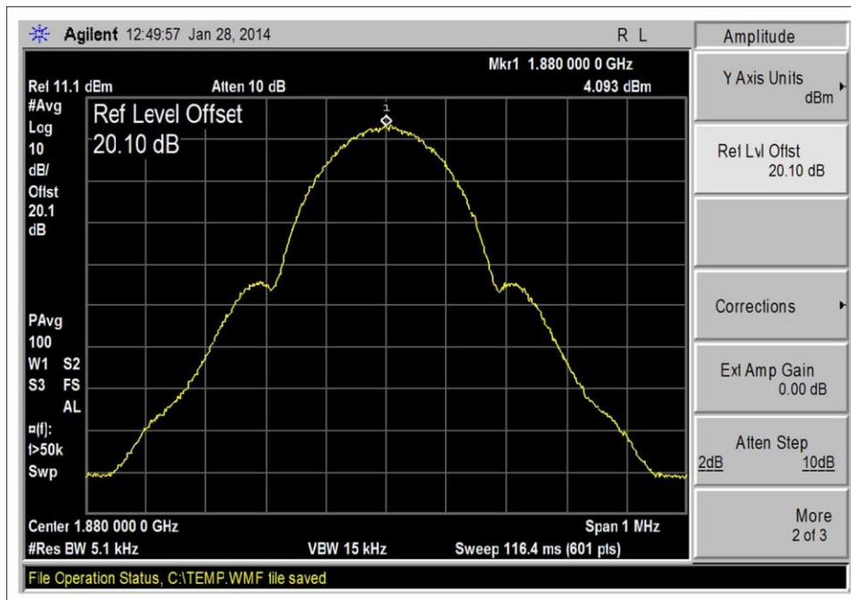
GSM_UL 1850-1910_Output
