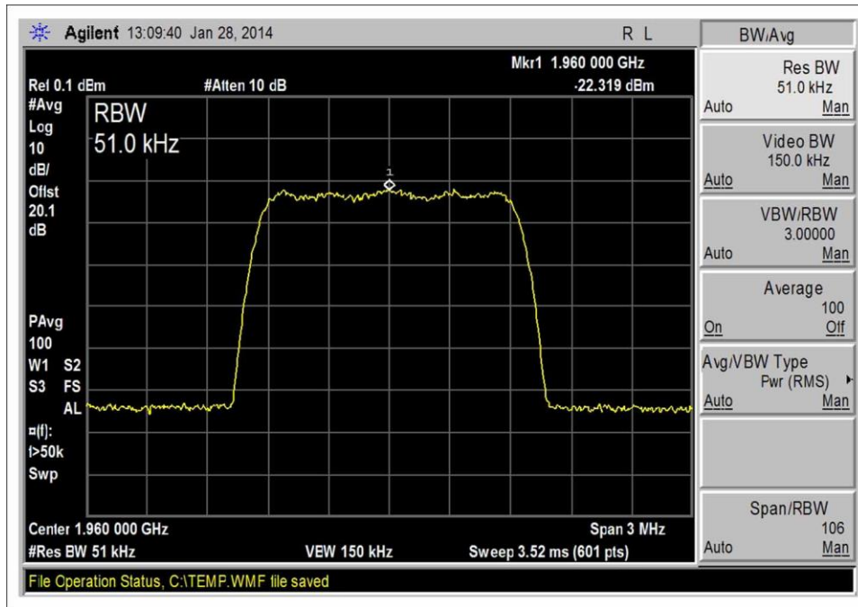
CDMA_DL 1930-1990_Output
