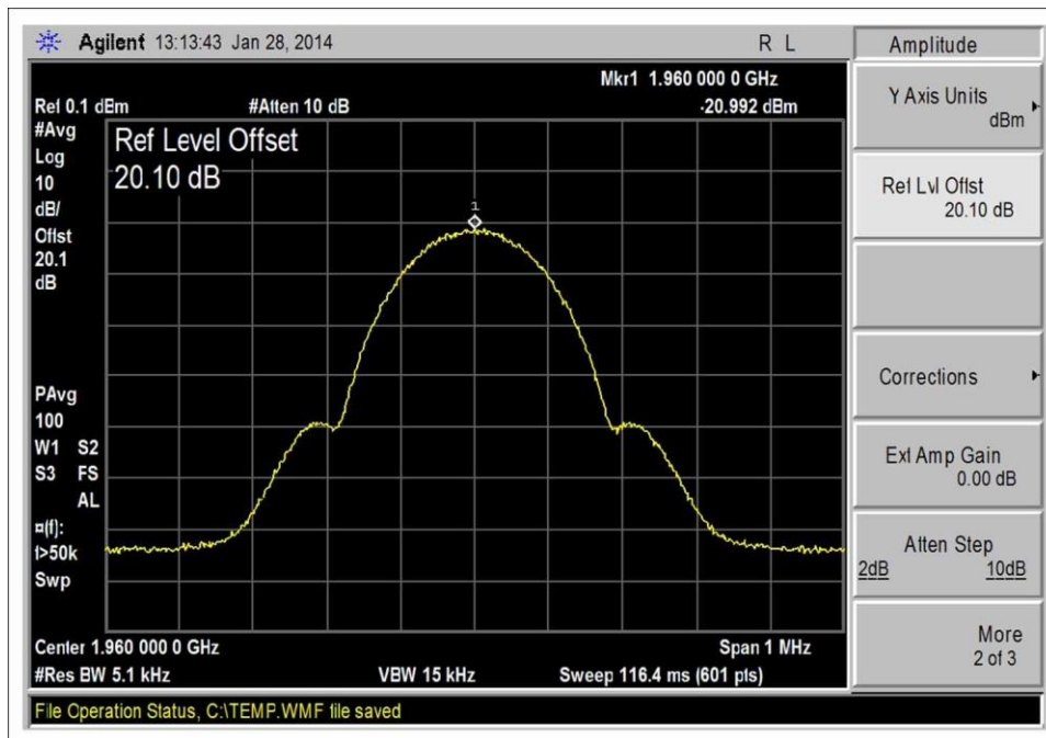
GSM_DL 1930-1990_Output
