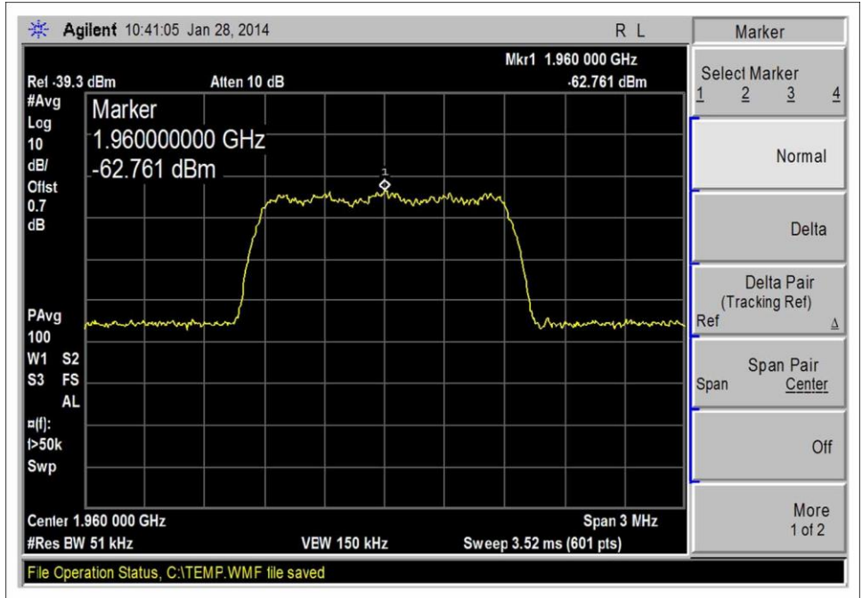
CDMA_DL 1930-1990_Input
