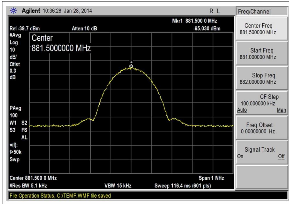
GSM_DL 869-894_Input
