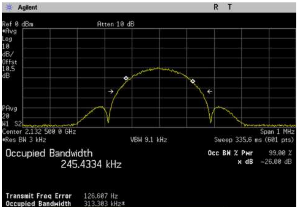
7.10 OBW-In_DL_2110-2155_EDGE_ 2132.5MHz
