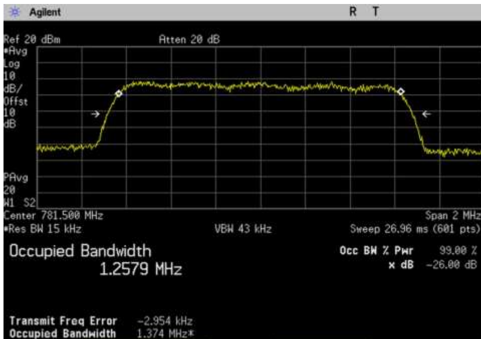
7.10 OBW-Out_UL_776-787_CDMA_781.5MHz
