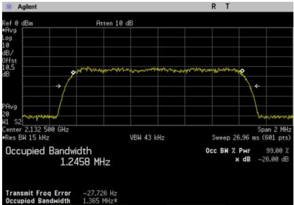
7.10 OBW-In_DL_2110-2155_CDMA_ 2132.5MHz
