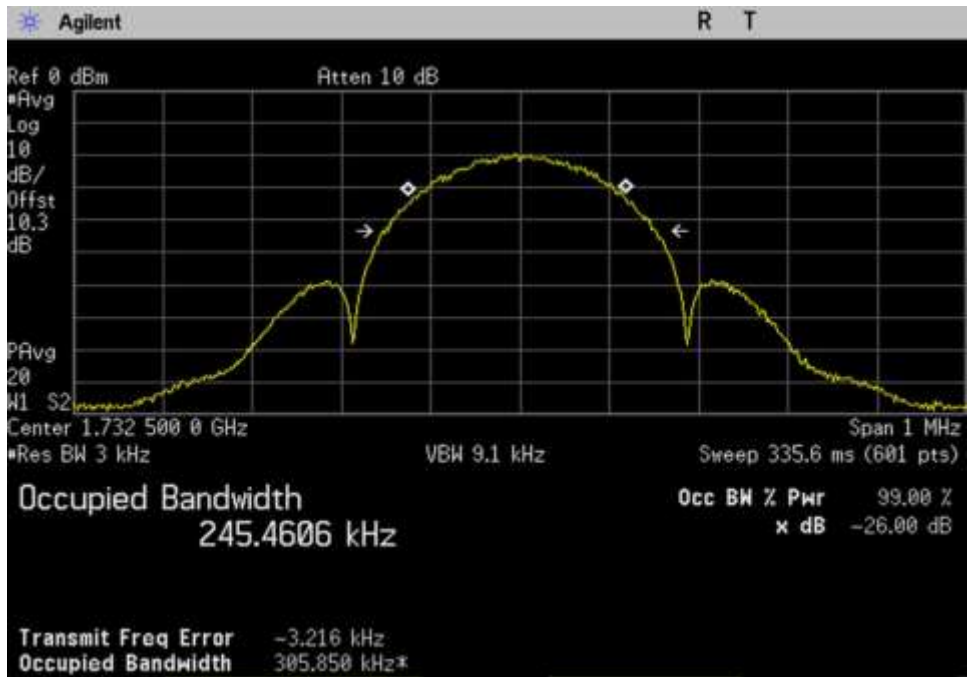
7.10 OBW-In_UL_1710-1755_EDGE_1732.5MHz
