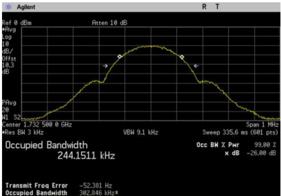
7.10 OBW-In_UL_1710-1755_GSM_1732.5MHz
