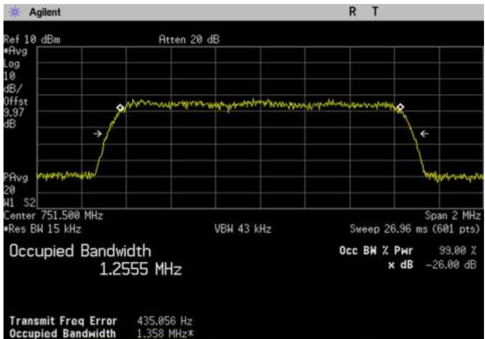
7.10 OBW-Out_DL_746-757_CDMA_751.5MHz
