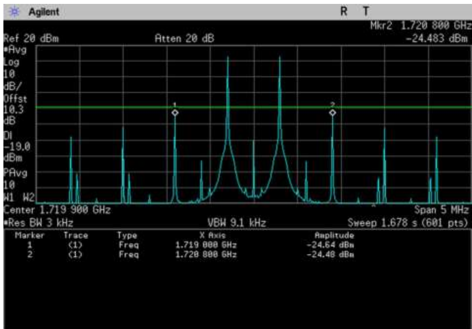
7.4 Intermod_UL_1710-1755_ 1719.9MHz
