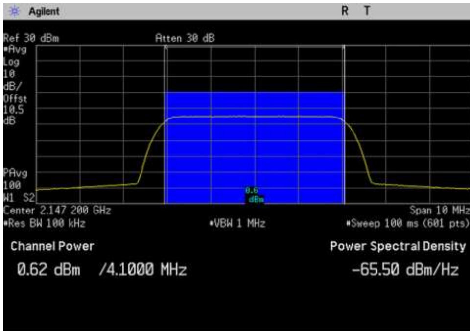
7.2-7.3 Power Gain_DL_2110-2155_AWGN_Max_2147.2MHz
