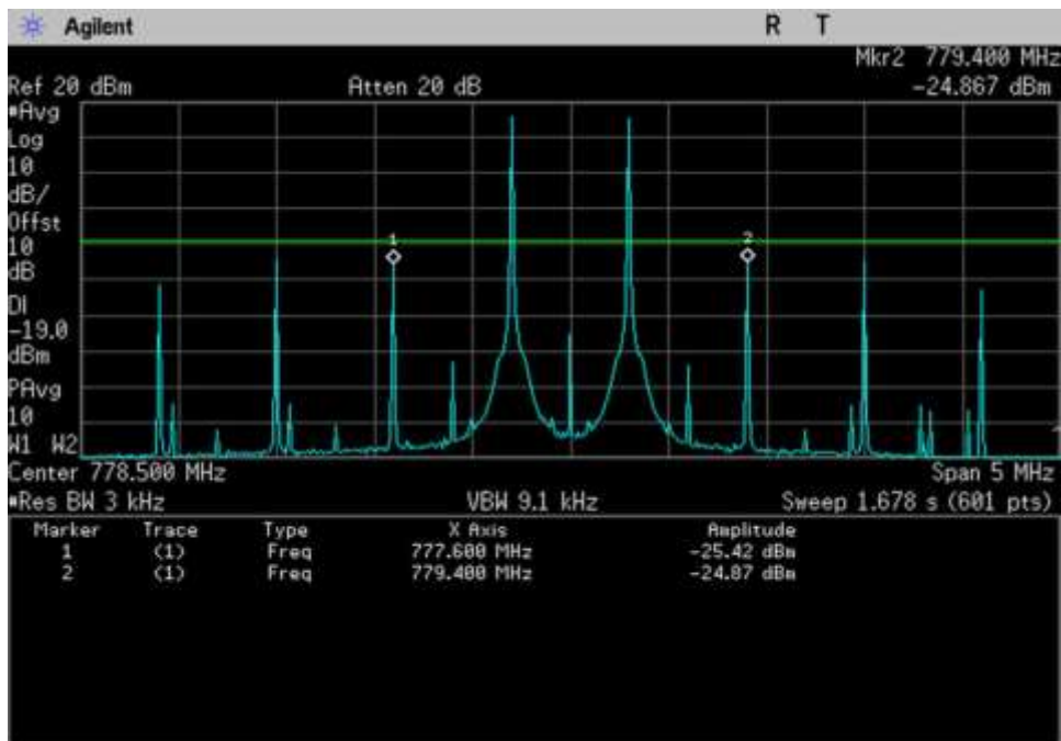
7.4 Intermod_UL_776-787_ 778.5MHz
