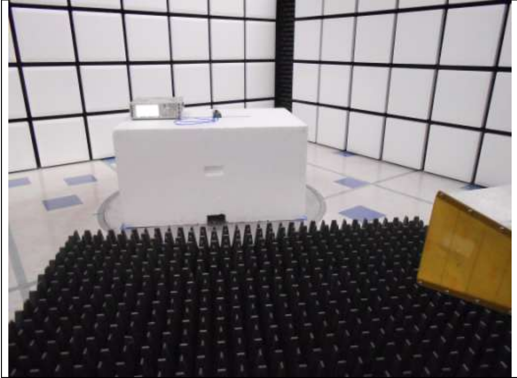
RF Radiated (EUT at 3 meters)
