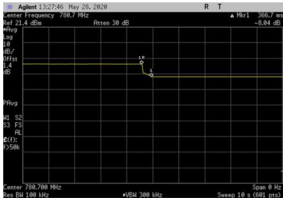
UL_776-787_ 780.7MHz_Timing
