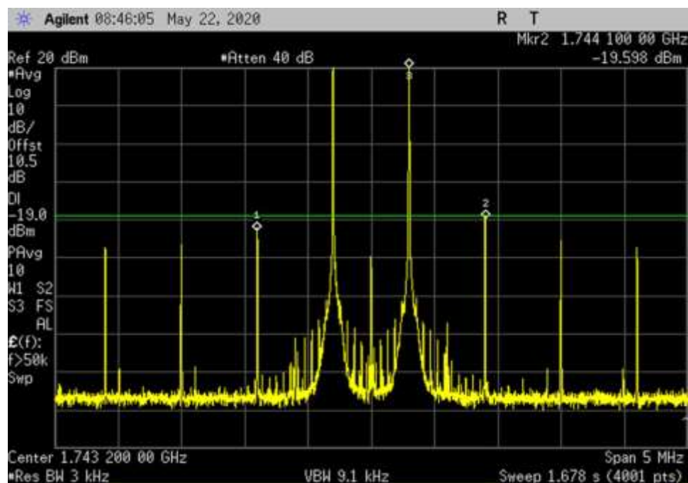
UL_1710-1755_1743.2MHz
