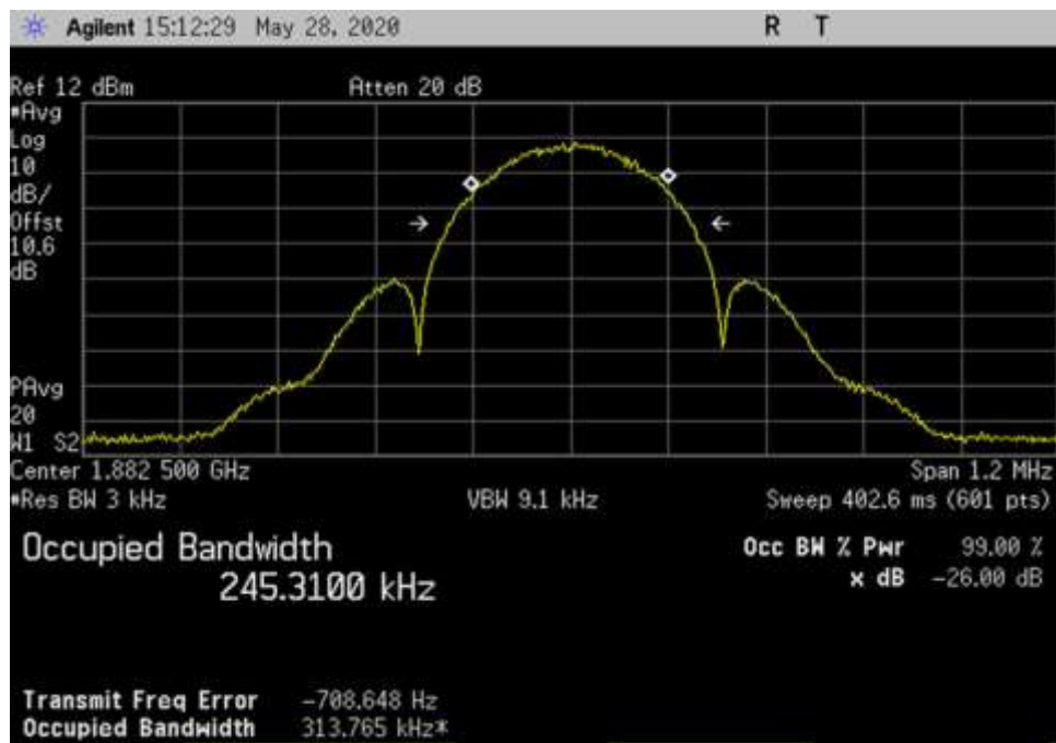
UL_1850-1915_EDGE_1882.5MHz
