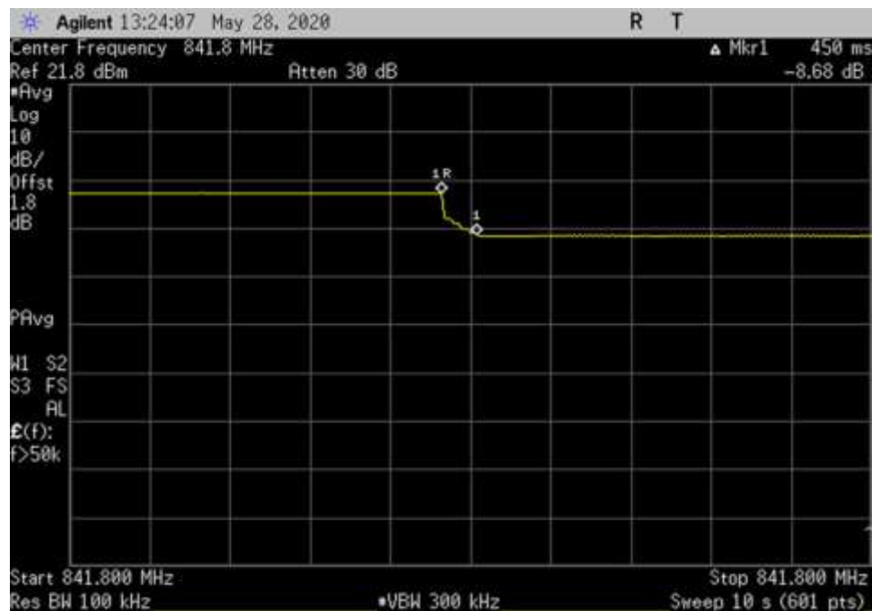
UL_824-849_ 841.8MHz_Timing
