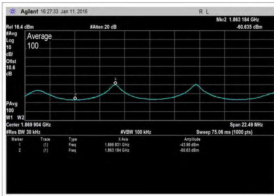
UL-1850-1915-AWGNL+2
