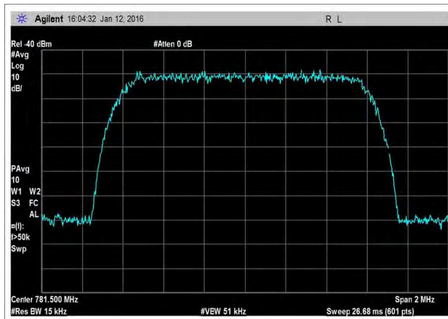
7.10_OBW_UL_776-787MHz_CDMA
