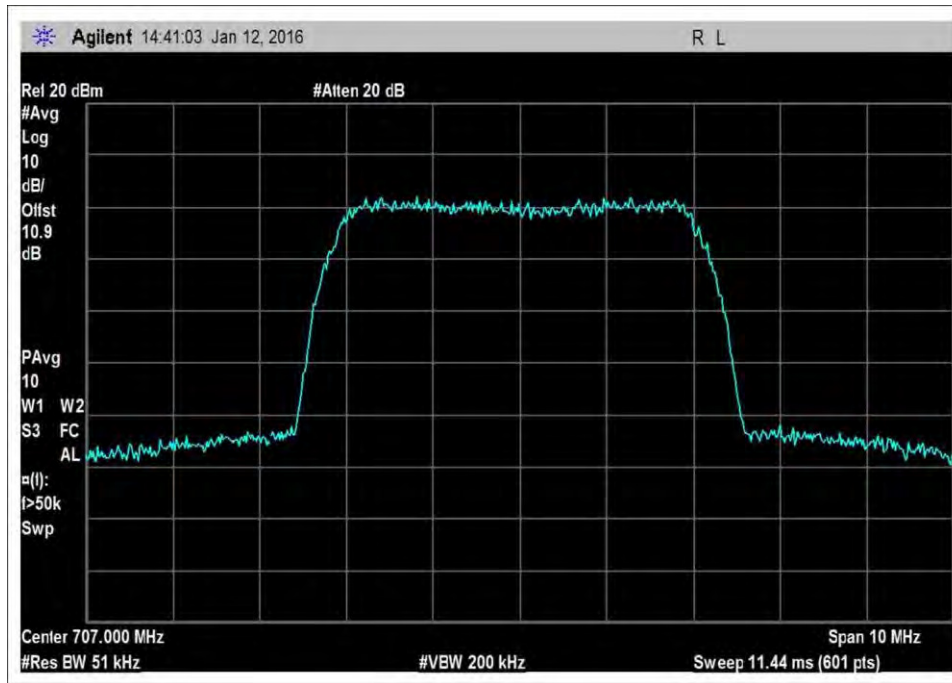
7.10_OBW_UL_698-716MHz_WCDMA
