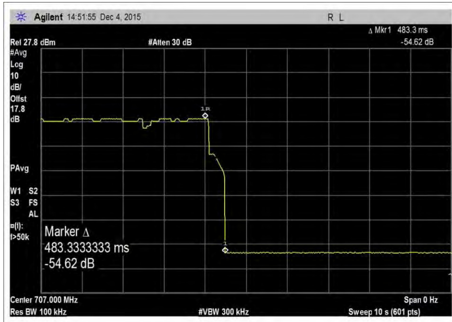
7.9.2_VarULGainTiming_UL_698-716MHz
