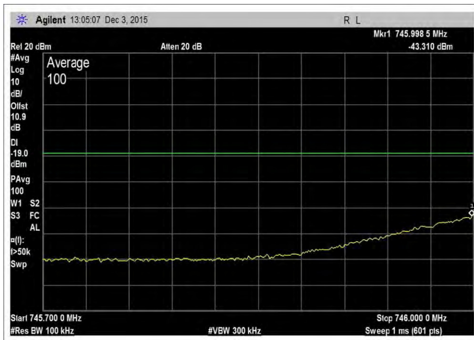
7.5_OBE_DL_746-757MHz_L_PreAGC
