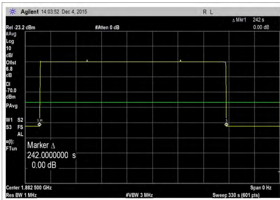
7.8_Inactivity_UL_1850-1915MHz
