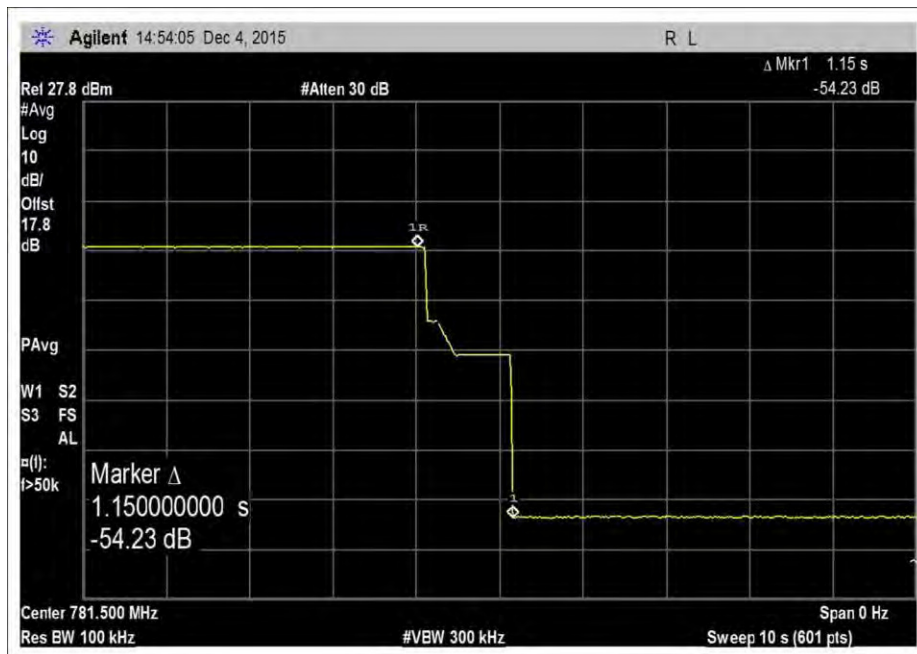
7.9.2_VarULGainTiming_UL_776-787MHz
