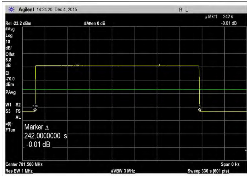
7.8_Inactivity_UL_776-787MHz
