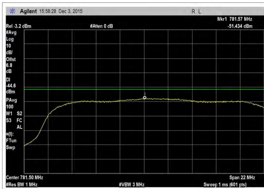
7.7_Noise_UL_776-787MHz
