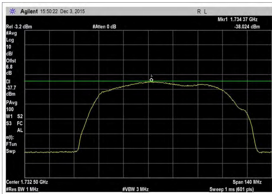
7.7_Noise_UL_1710-1755MHz-Zoom
