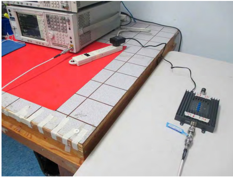
7.8 Test Setup
