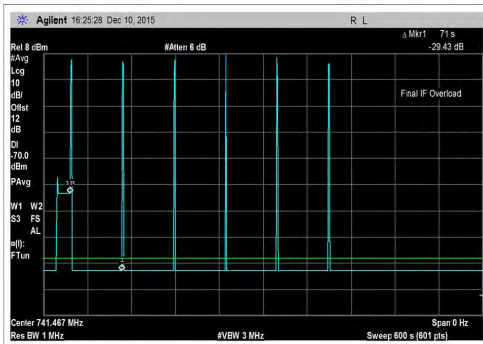
7.11_osc_DL-728-746MHz-600sec
