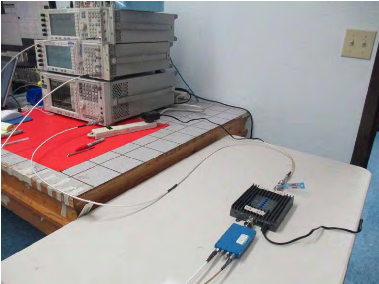
7.4 Test Setup
