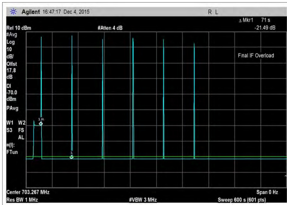
7.11_osc_UL-698-716MHz-600sec
