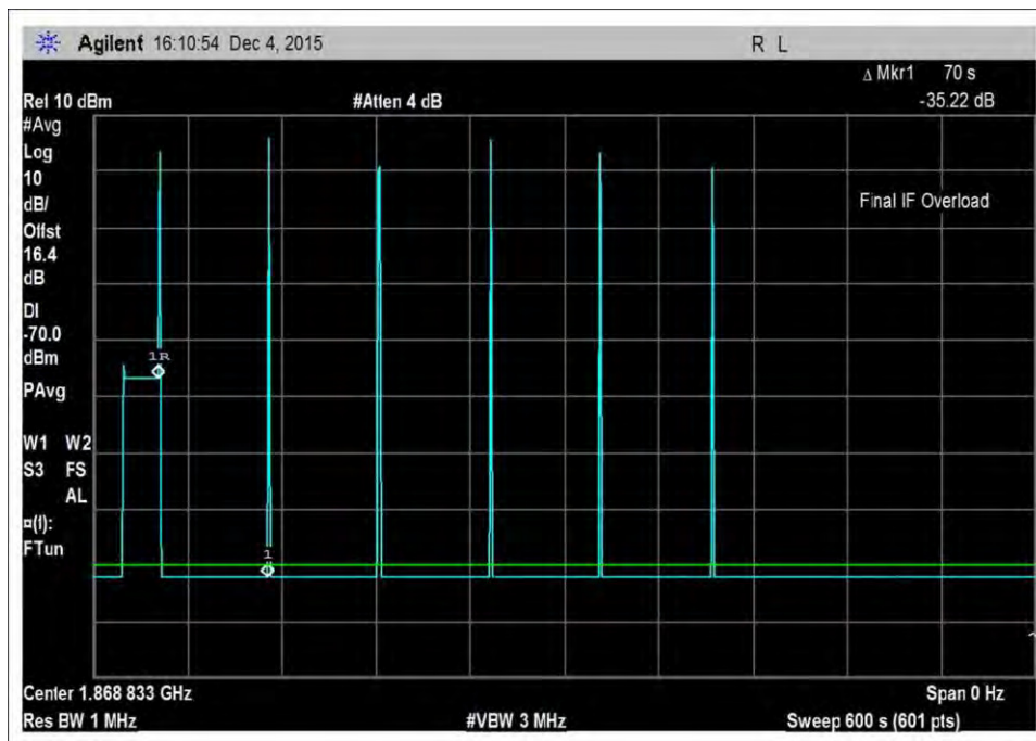
7.11_osc_UL-1850-1915MHz_600sec
