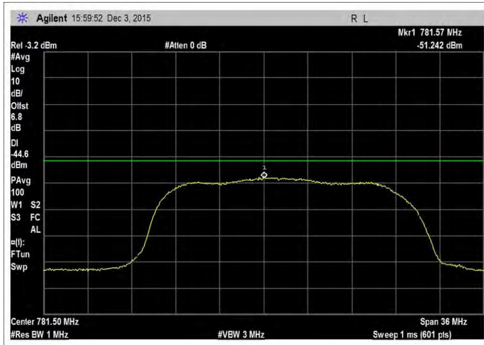
7.7_Noise_UL_776-787MHz-Zoom
